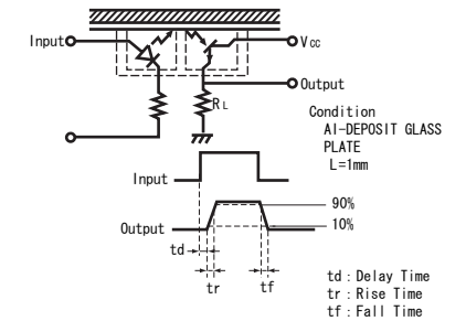
*2 Method of measuring position detection characteristic
